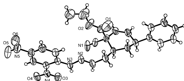
Figure 1. ORTEP plot of the 2,4-dinitrobenzenehydrozone derivative of enantiopure 3q drawn with ellipsoids at 30% probability
